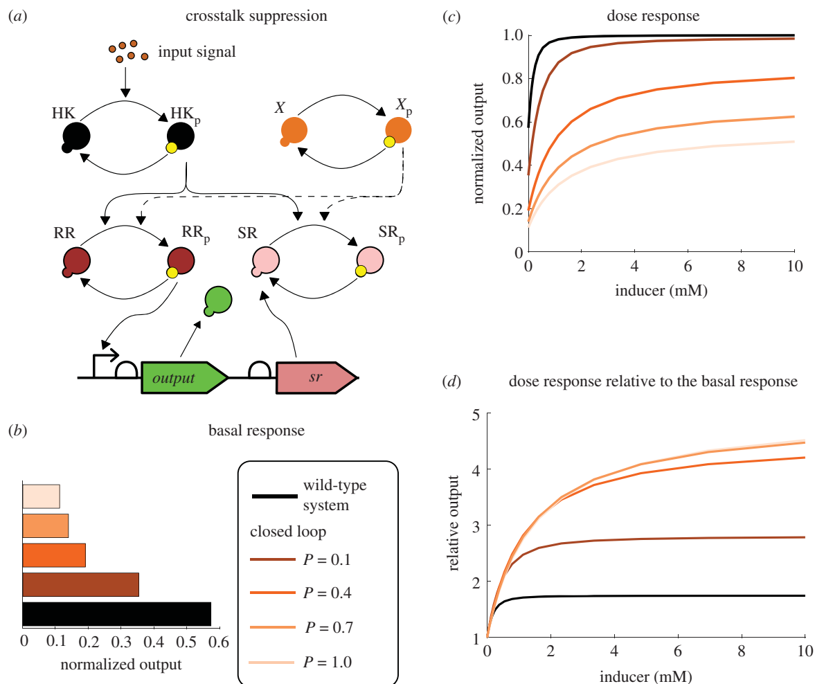
Figure 9. (a) A schematic depiction of a two-component system with the dichotomous feedback architecture and crosstalk with another histidine kinase X . (b) Basal response ( [I] = 0 [mM]) of the wild-type and the closed-loop systems with various feedback strengths divided by the maximal response. (c) Dose–response curves of the wild-type and the closed-loop systems with various feedback strengths divided by the maximal response. (d) Dose–response curves of the wild-type and the closed-loop systems with various feedback strengths each divided by their basal response. The curves for P = 1 and P = 0.7 are indistinguishable by the naked eye. These simulations suggest that dichotomous feedback architecture can reduce crosstalk in the system.
